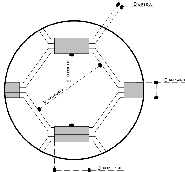
DRAWING : Hex Mesh Belt
