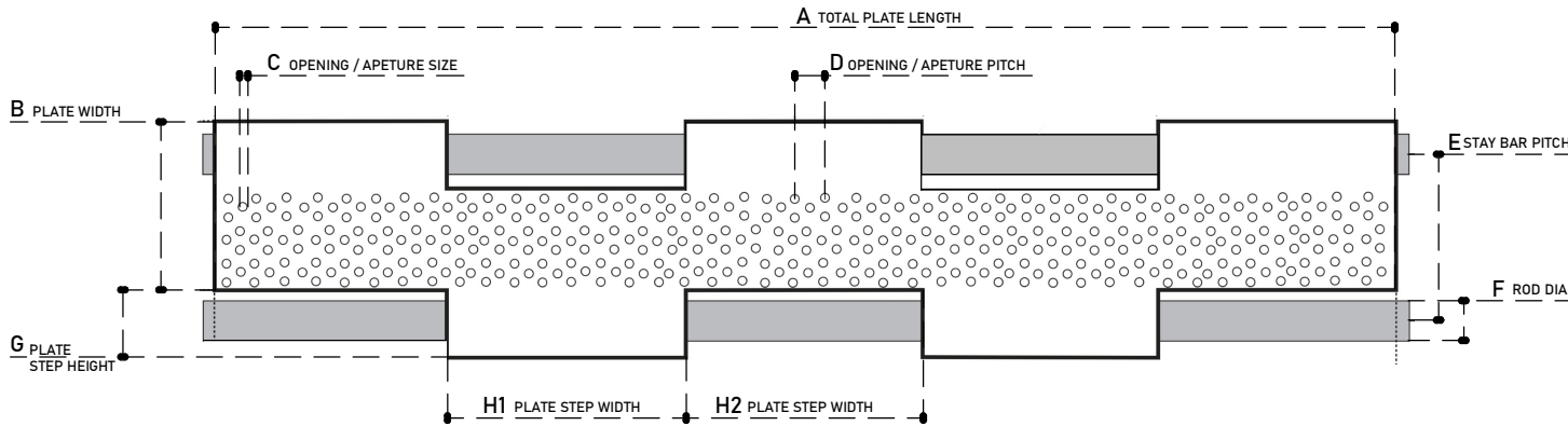
DRAWING : Plate Belt - with Chain
